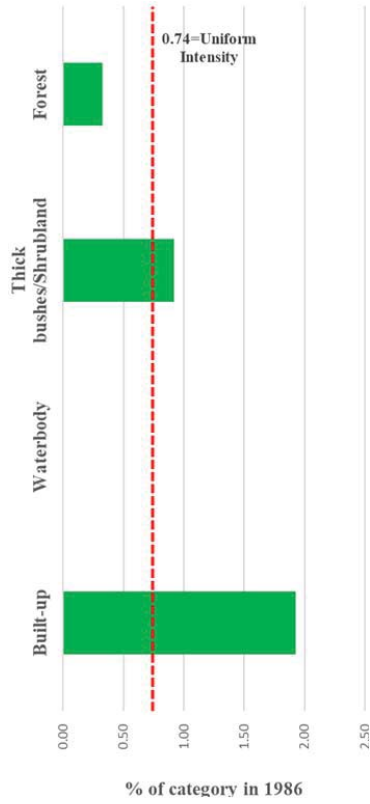
Fig. 13 (a) Transition to Agriculture in 1986-2002
