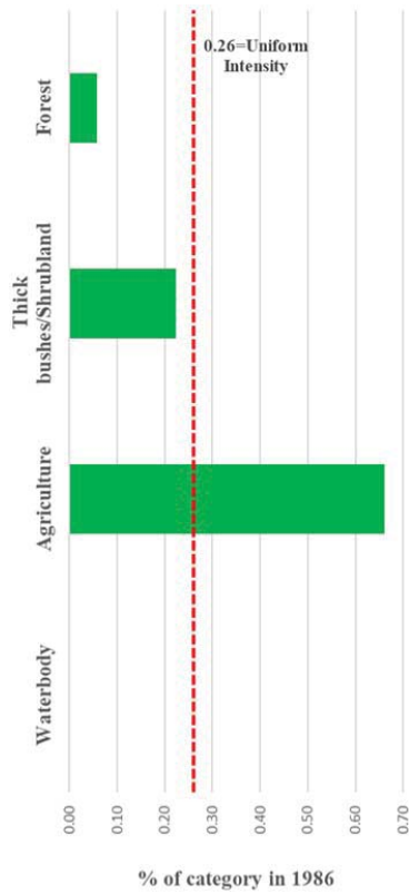
Fig. 9 (a) Transition to Built-up in 1986-2002
