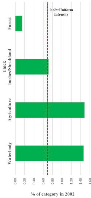
Fig. 11 (a) Transition to Built-up in 2002-2017
