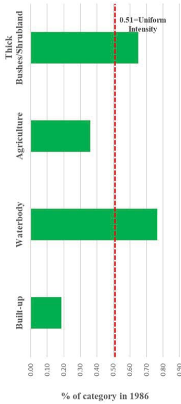
Fig. 17 (a) Transition to forest in 1986-2002
