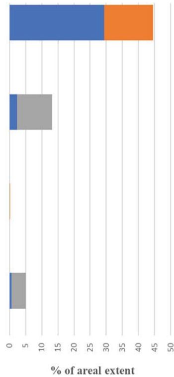
Fig. 18 (b) Hypothetical error of commission/omission Though agriculture gained from built-up in the first interval, it lost heavily to built-up in the same period, hence, the shrunken of -8.44%. But agriculture recorded 52.07% increase mainly due to transitions from thick bushes, which was large
