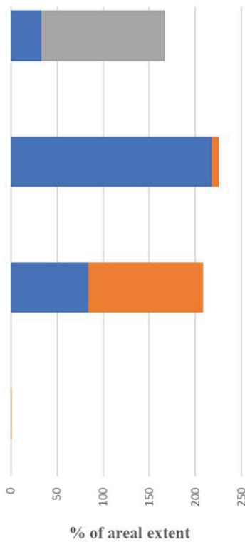
Fig. 11 (b) Hypothetical error of commission/omission
