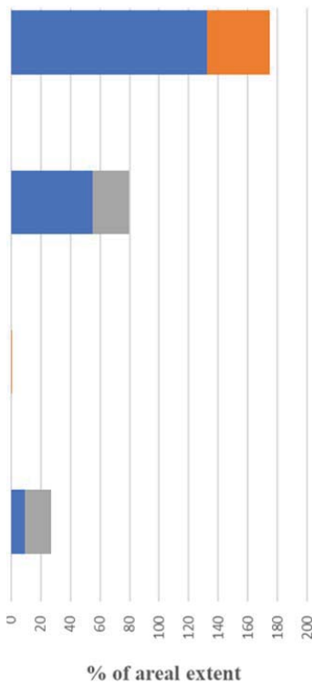
Fig. 17 (b) Hypothetical error of commission/omission
