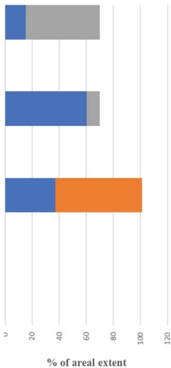
Fig. 9 (b) Hypothetical error of commission/omission
