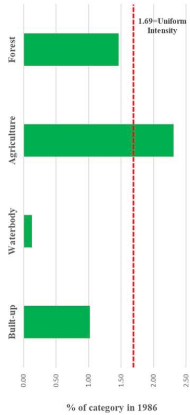
Fig. 14 (a) Transition to Thick bushes/shrubland in 1986-2002
