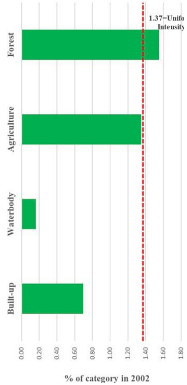
Fig. 16 (a) Transition to Thick bushes/shrubland in 2002-2017
