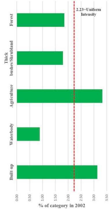
Fig. 7 (a) Loss intensity in 1986-2002
