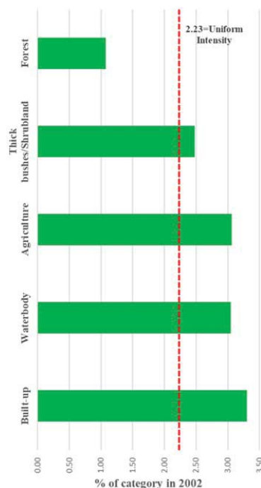
Fig. 5 (a) Gain intensity in 1986-2002
