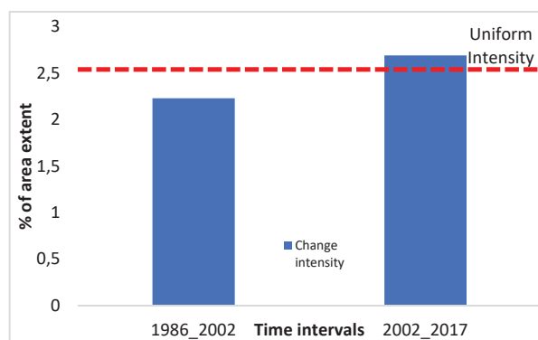
Fig. 3 Hypothetical uniform annual change between 1986-2002 and 2002-2017
