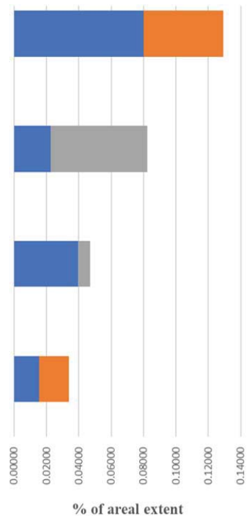
Fig. 10 (b) Hypothetical error of commission/omission
