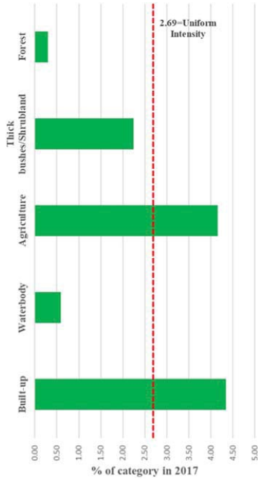
Fig. 6 (a) Gain intensity in 2002-2017
