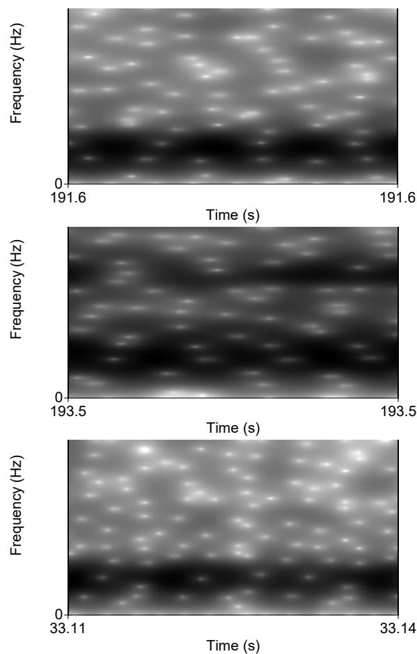
Fig. 8 Contour spectrogram of sound a
