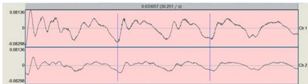
Fig. 5 The second monozygotic twin
