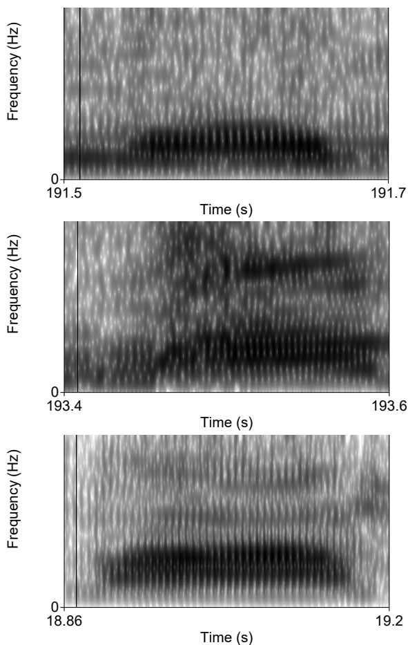
Fig. 9 Contour spectrogram of the word “mam”
