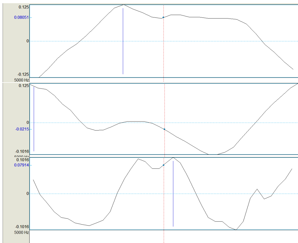
Fig. 6 One period in sound m
