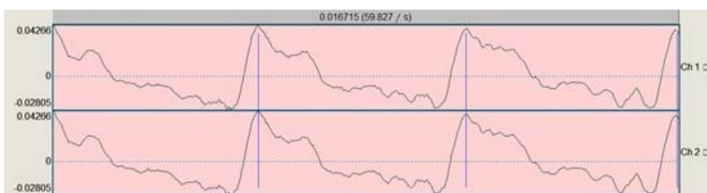
Fig. 4 The first monozygotic twin
