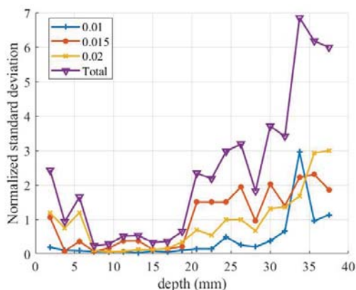
Fig. 4 Normalized standard deviation of measurement versus depth
