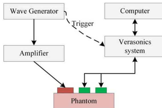
Fig. 2 The circular element and two rectangular elements are used to generate and track shear waves respectively
