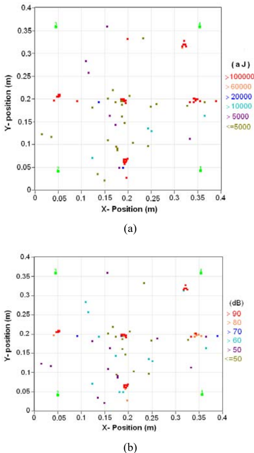
Fig. 11 Planar location of events with (a) Absolute energy (atto joules) (b) Amplitude (dB)
