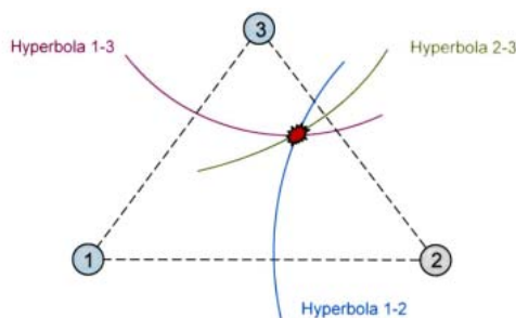
Fig. 6 2D location with three sensors [2]
