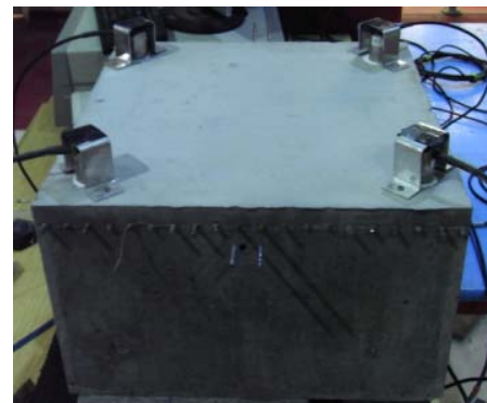
Fig. 9 Photograph of specimen with sensors setup
