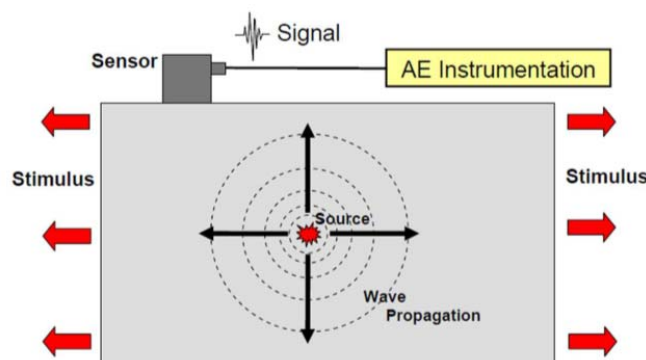
Fig. 1 AE method [4]
