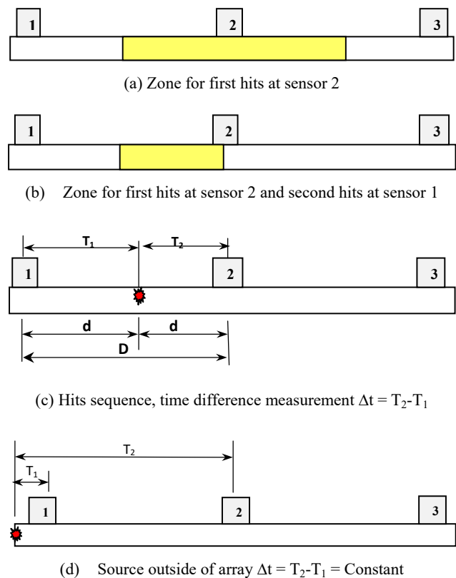
Fig. 4 Linear location using TOA theory [15]
