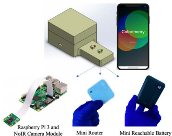
Fig. 1 A schematic of lightbox and its components wirelessly controlled by cellphone
