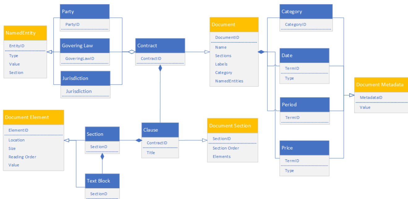
Fig. 5 The Extension Model Definition for Contracts
