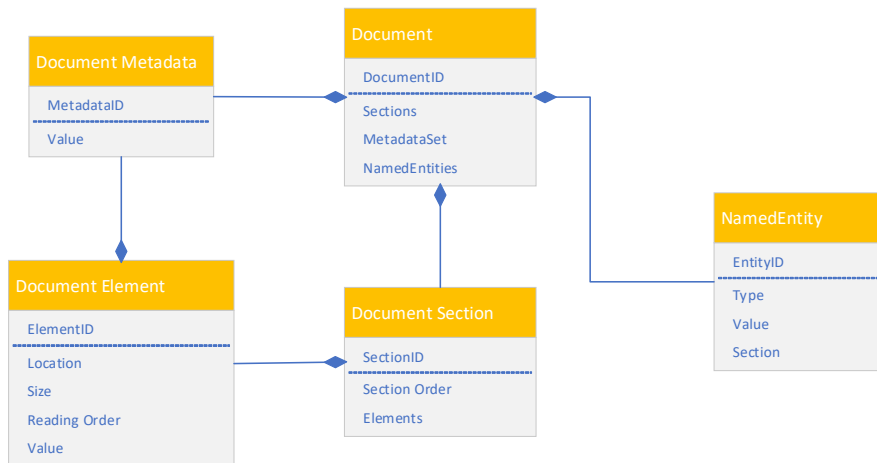
Fig. 2 The Core Model Definition of DocPro
