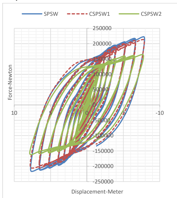
Fig. 7 Hysteresis curve in models; (a) SPSW, (b) CSPSW1 and (c) CSPSW2 under cyclic load
