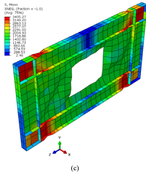
Fig. 4 Von Mises Stress in models; (a) SPSW, (b) CSPSW1 and (c) CSPSW2 under cyclic load
