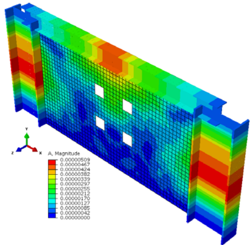
Fig. 14 Acceleration of SPSW2 model under Kobe earthquake
