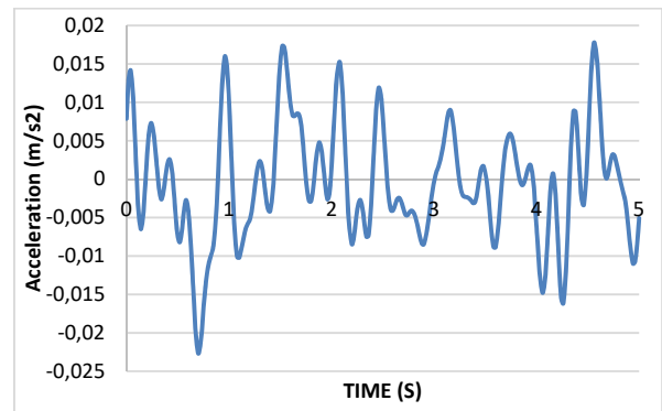
Fig. 4 Kobe earthquake diagram (Acceleration-time)
