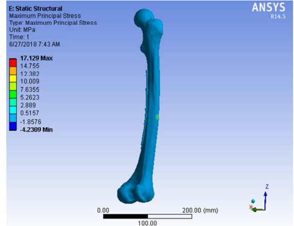
Fig. 6 (a) Maximum principal stress in clinical setup
