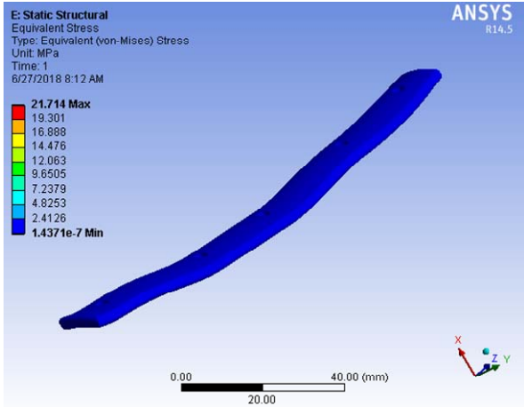
Fig. 5 (c) Von-Mises stress distribution in implant
