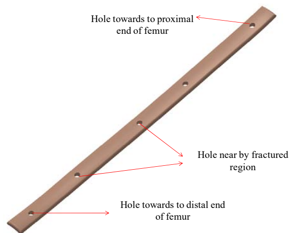
Fig. 3 Customized implant designed for fractured bone
