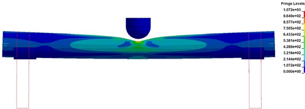
Fig. 6 Stress Distribution on FE model of the impacted area
