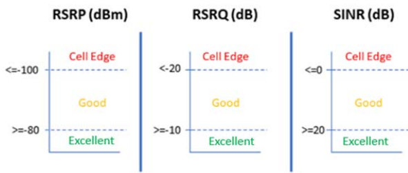
Fig. 3 Power Levels RSRP, RSRQ and SINR [15]
