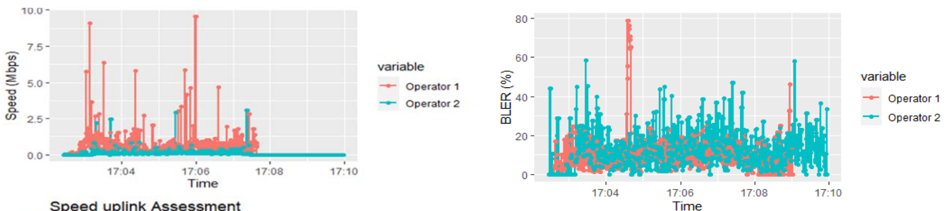
Fig. 20 BLER measurement scenario 3
