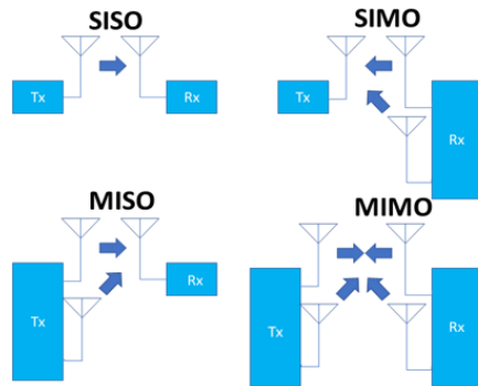
Fig. 2 MIMO antenna structure
