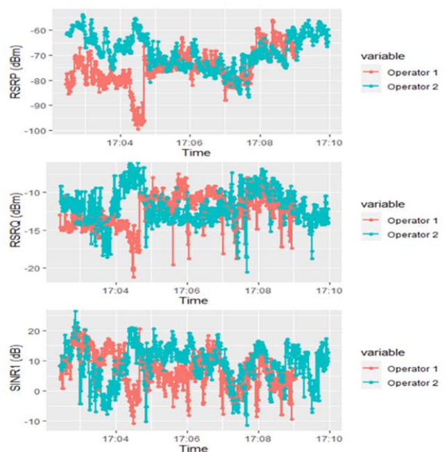
Fig. 17 RSRP, RSRQ, SINR1 measurement scenario 3
