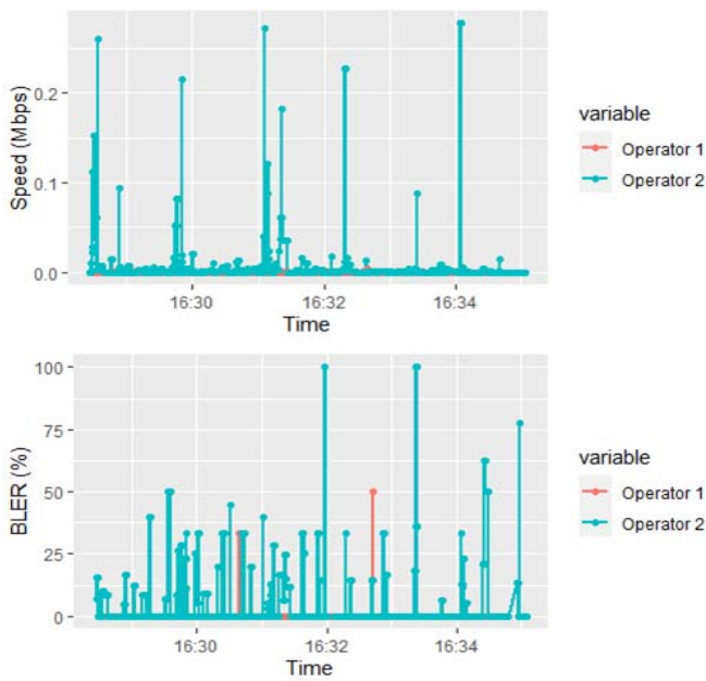
Fig. 13 Speed Downlink and BLER scenario 1
