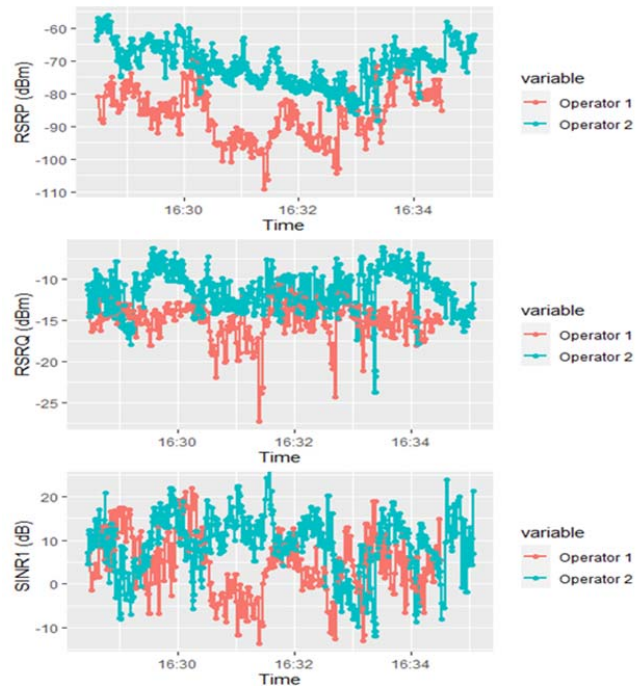
Fig. 11 RSRP, RSRQ and SINR1 measurements scenario 1
