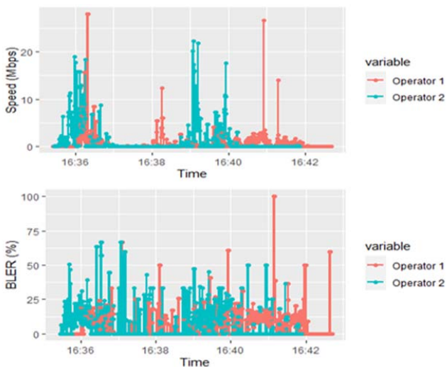
Fig. 16 Speed Downlink and BLER measurement scenario 2
