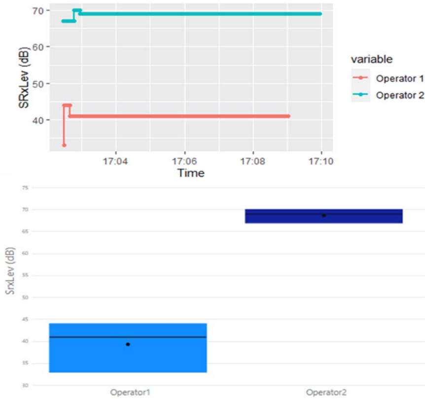
Fig. 18 SRxLev with bloxplot measurements scenario 3
