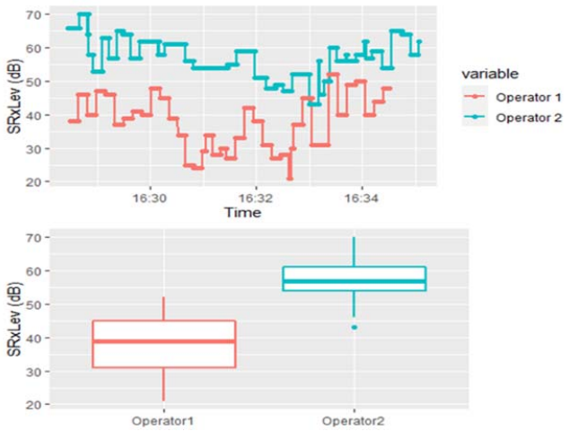
Fig. 12 SRxLev with boxplot measurements scenario 1
