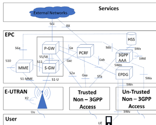
Fig. 1 Basic LTE architecture
