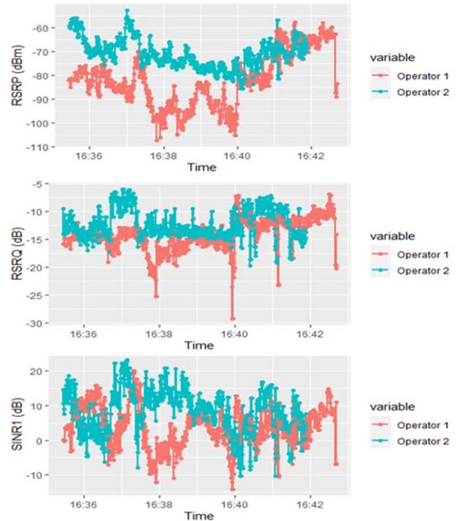
Fig. 14 RSRP, RSRQ and SINR1 measurements scenario 2
