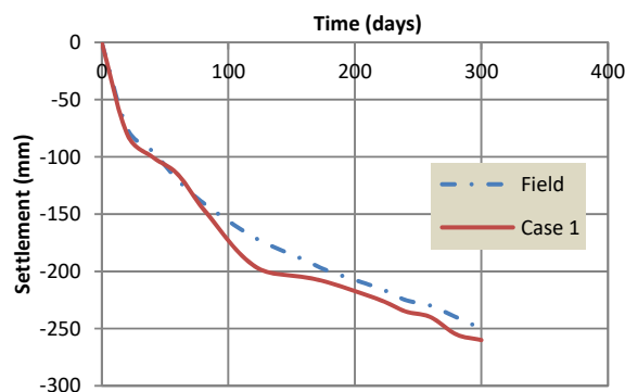
Fig. 3 The estimated and measured settlement versus time results at the center of railway
