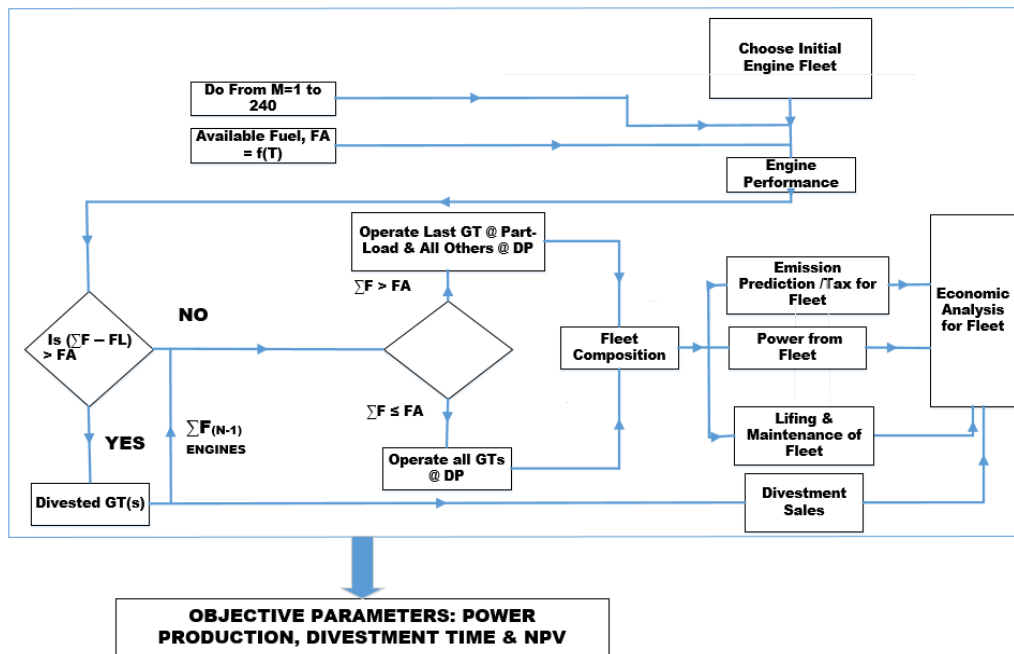
Fig. 2 TERA Methodology for Associated Gas Utilisation (Baseline)
