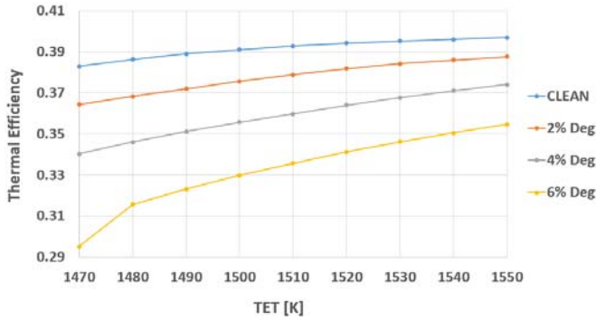
Fig. 10 TET (in K) against Thermal Efficiency
