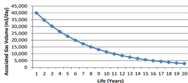
Fig. 1 Associated Gas Decline over 20 Years Period [1]
