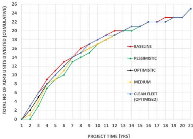
Fig. 4 Optimised Engine Units' Best Divestment Time & the Effect of Gas Turbine Degradation on Divestment Time
