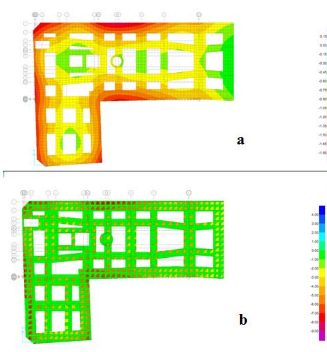
Fig. 5 The status of stresses below the foundation under the service load (a) before the improvement, (b) after the improvement
