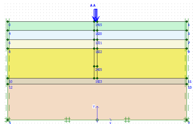
Fig. 7 Numerical modeling in PLAXIS software for a column JG
