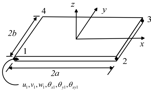
Fig. 2 A conforming rectangular element with six degrees of freedom (u_i, v_i, w_i, \theta_{xi}, \theta_{yi}, \theta_{xyi}) per node
