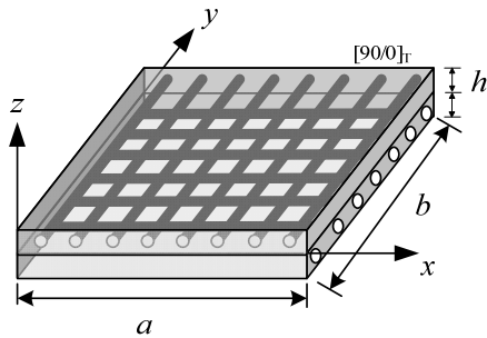
Fig. 8 Composite laminates with cross-ply stacking sequence.
