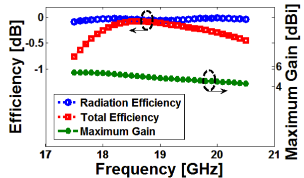
Fig. 6 Fundamental properties of the single-element antenna
