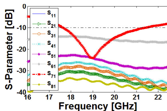
Fig. 9 S parameters of the designed 5G antenna
