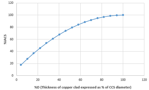
Fig. 4 % IACS of CCS against Copper Clad Thickness
