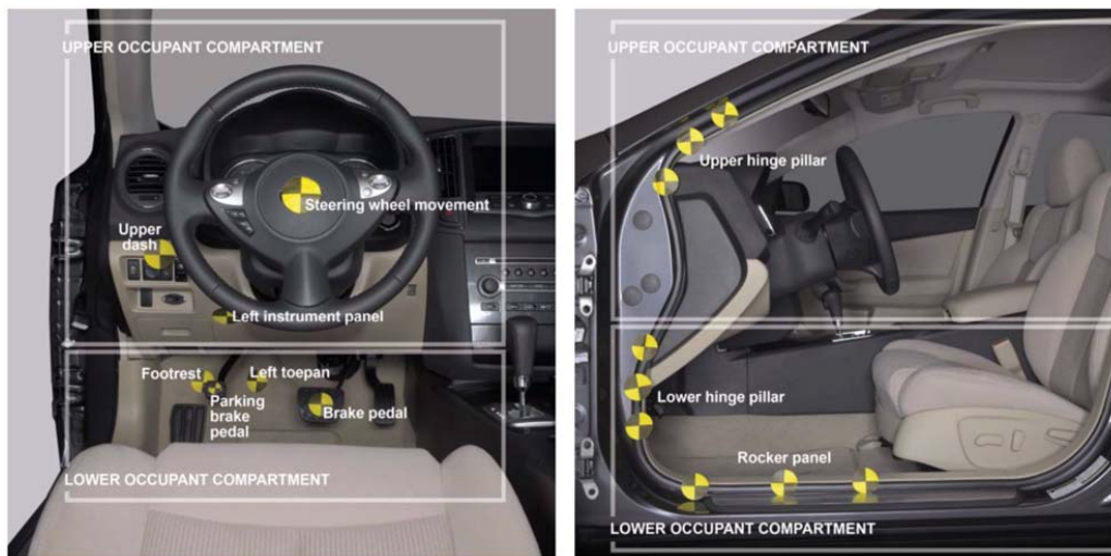
Fig. 3 Locations for Measuring Vehicle Intrusion
