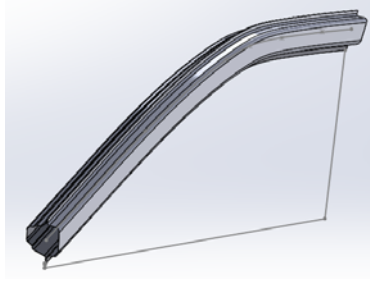
Fig. 10 CAD Model of 2015 Camry A-Pillar
