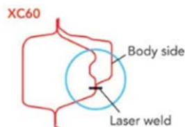
Fig. 8 2012 Volvo XC60 A-Pillar Cross-Section
