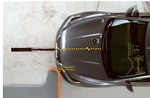
Fig. 2 Driver-side Small Overlap Frontal Test Configuration
