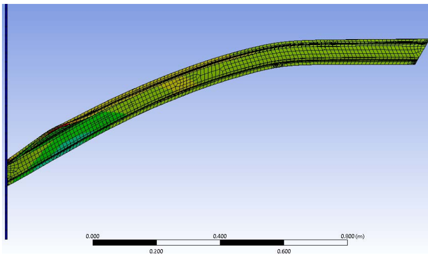
Fig. 14 ANSYS Simulation of 2015 Camry A-Pillar
