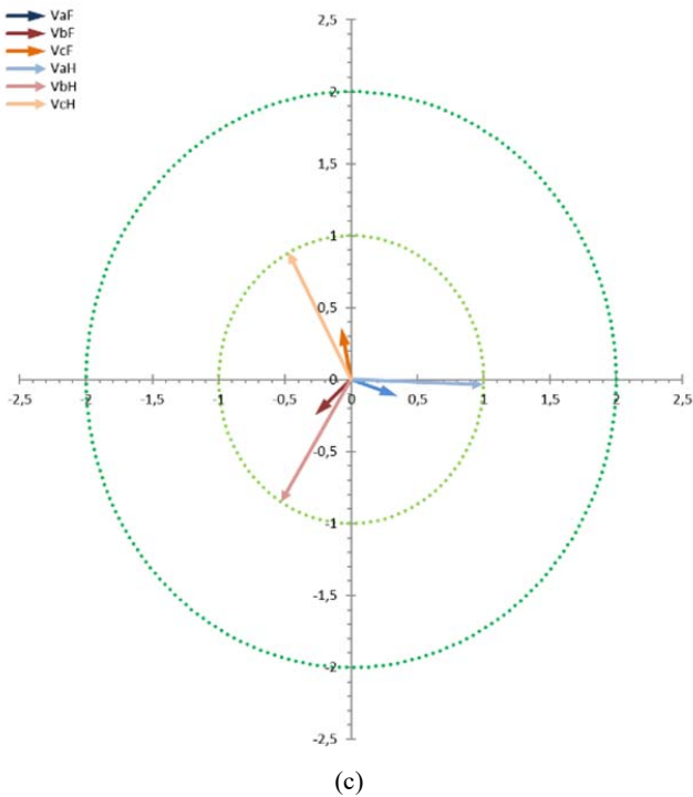
Fig. 9 Cases (a) 1-1-3-3ph-1, (b) 1-1-3-3ph-2, (c) 1-1-3-3ph-5
