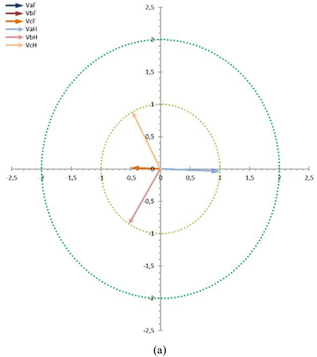
Fig. 5 Cases (a) 1-1-3-1phN-3, (b) 1-1-3-1phN-4, (c) 1-1-3-1phN-5
