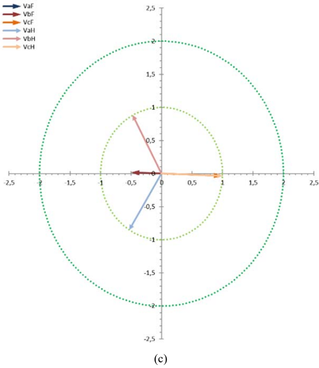
Fig. 11 Cases (a) 5-7-1-2ph-1, (b) 5-7-1-2ph-3, (c) 5-7-1-2ph-5
