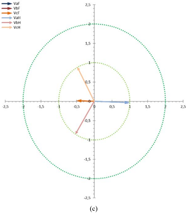
Fig. 6 Cases (a) 1-1-1-2ph-1, (b) 1-1-1-2ph-3, (c) 1-1-1-2ph-5
