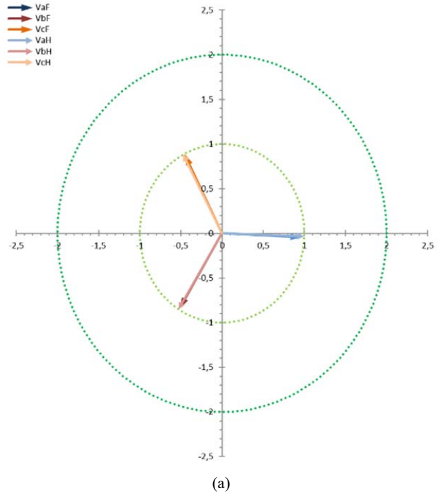
Fig. 3 Cases (a) 1-1-1-phN-1, (b) 1-1-1-phN-2, (c) 1-1-1-phN-4
