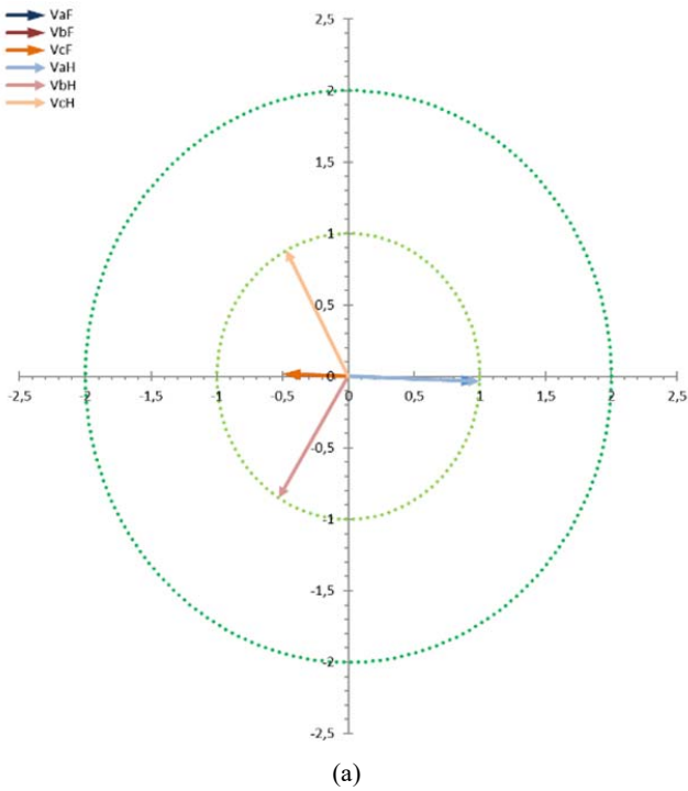
Fig. 11 Cases (a) 5-7-1-2ph-1, (b) 5-7-1-2ph-3, (c) 5-7-1-2ph-5
