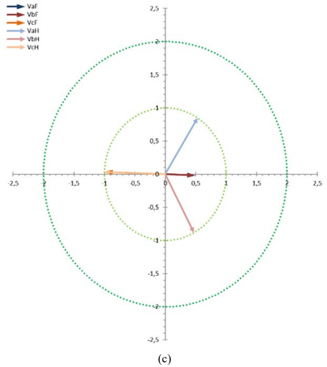
Fig. 12 Cases (a) 11-5-1-2ph-1, (b) 11-5-1-2ph-3, (c) 11-5-1-2ph-5
