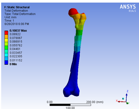
Fig. 7 Total deformation variation in clinical setup
