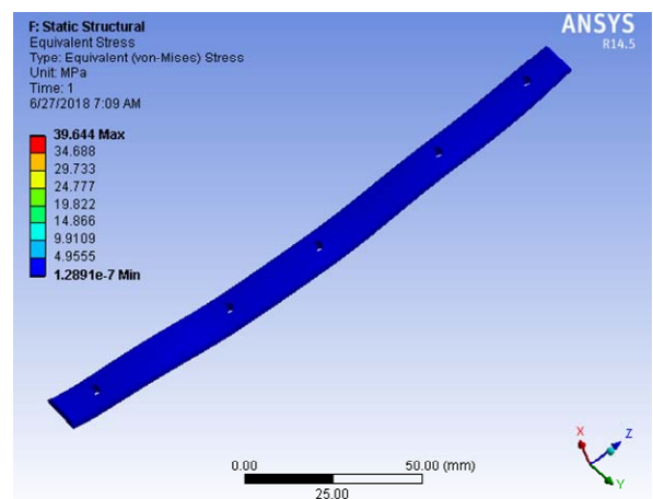
Fig. 5 (c) Von-Mises stress distribution in implant
