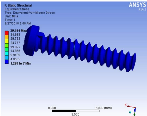
Fig. 5 (e) Von-Mises stress distribution in critical screw
