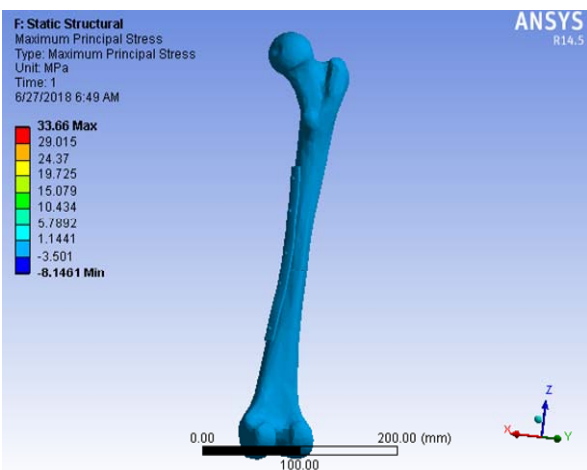
Fig. 6 (a) Maximum principal stress in clinical setup
