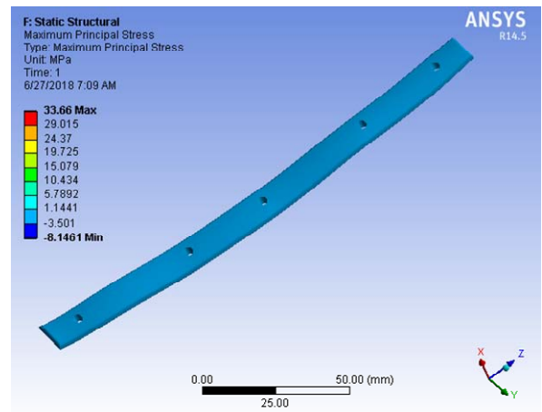
Fig. 6 (c) Maximum principal stress in implant
