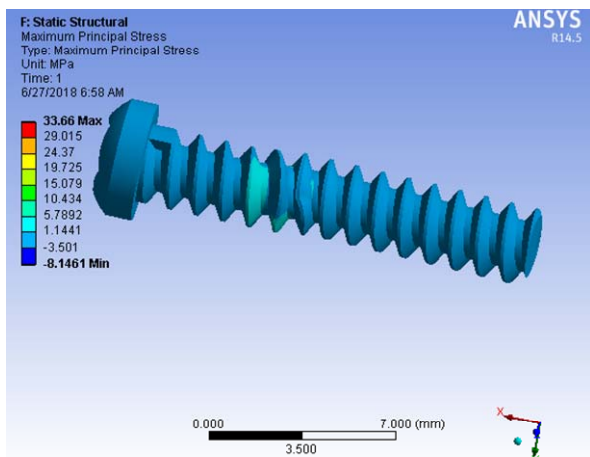
Fig. 6 (e) Maximum principal stress in critical screw
