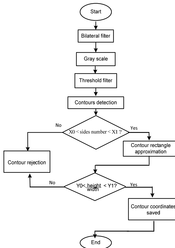
Fig. 1 NPL algorithm
