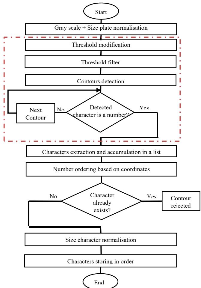
Fig. 4 CS algorithm
