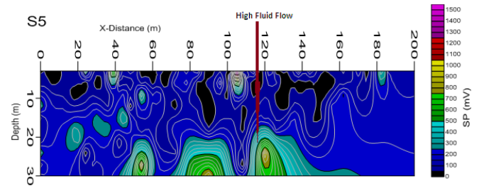
Fig. 7 SP 2D Section for Profile 5 (S5)
