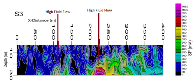
Fig. 5 SP 2D Section for Profile 3 (S3)
