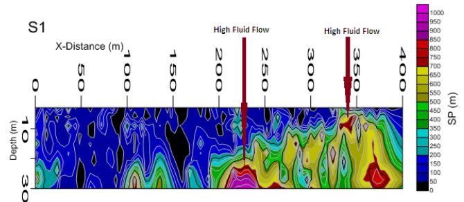
Fig. 3 2D Section for Profile 1 (S1)
