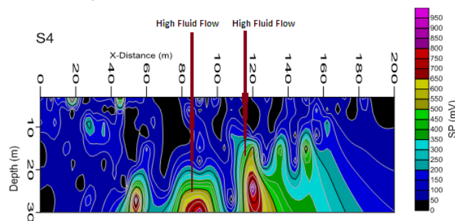
Fig. 6 SP 2D Section for Profile 4 (S4)
