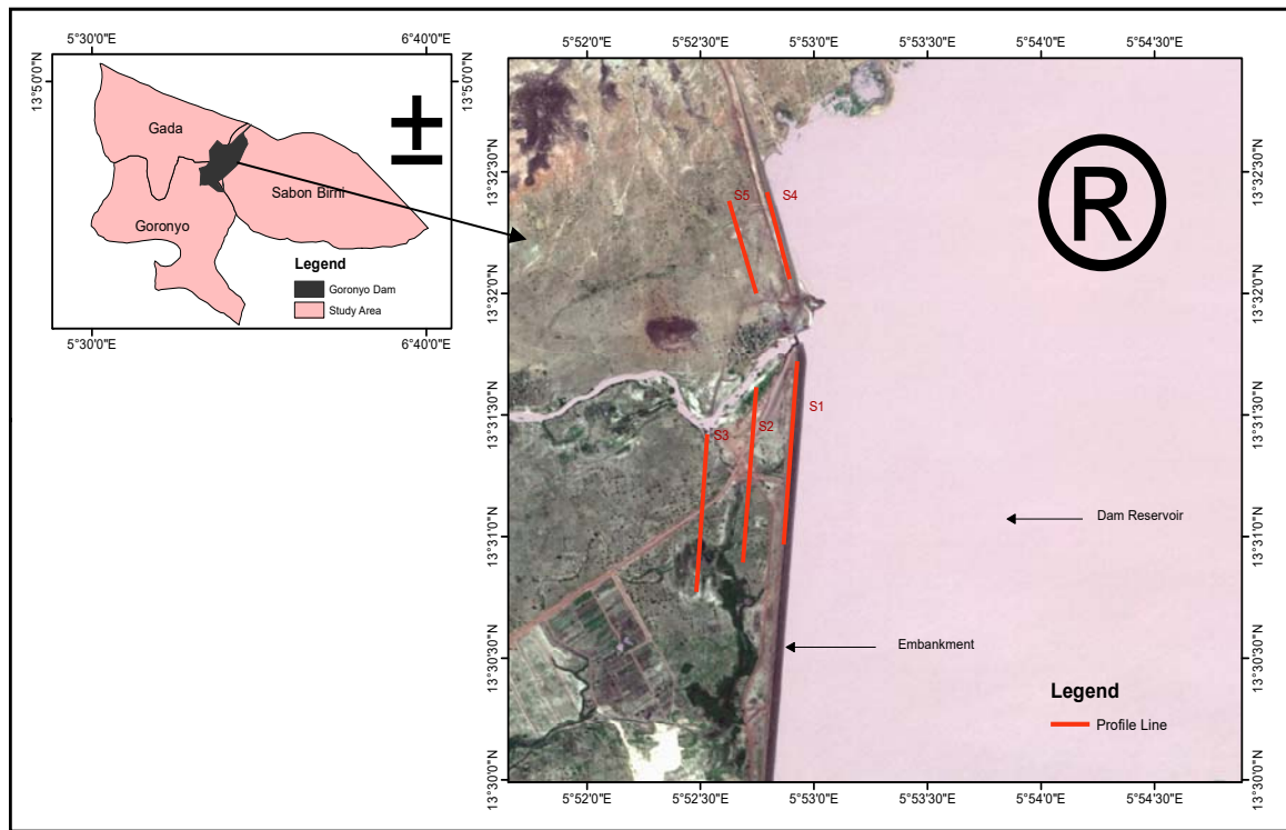
Fig. 2 Field Survey Layout Using Wenner Electrode Configuration
