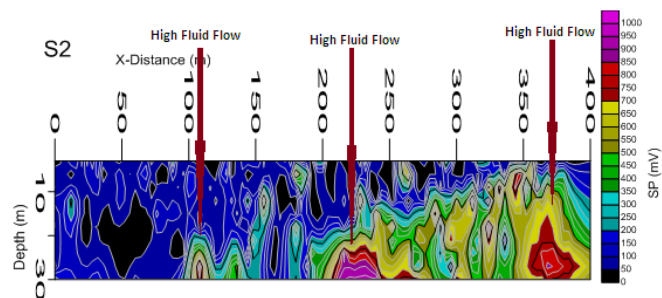
Fig. 4 SP 2D Section for Profile 2 (S2)
