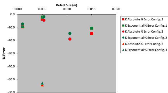
Fig. 18 Stress-Intensity Factor % Error for All Configurations-Thick Cylinder
