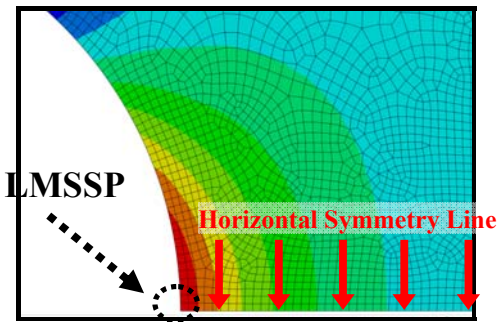
Fig. 5 LMSSP for Flat Plate with Circular Hole
