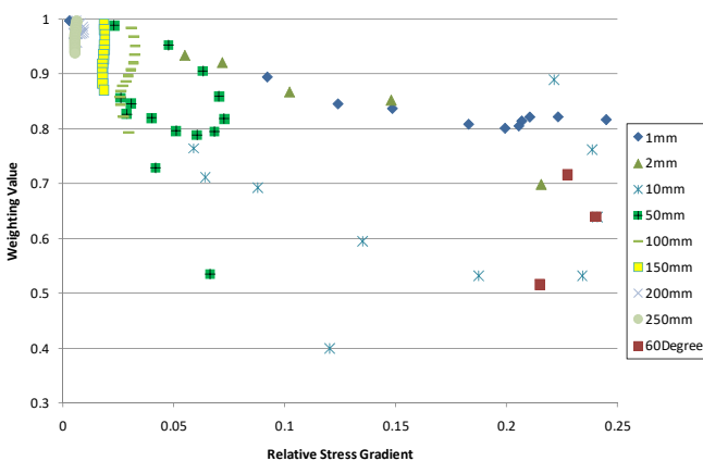
Fig. 20 Absolute Weighting Function Values for Notch
