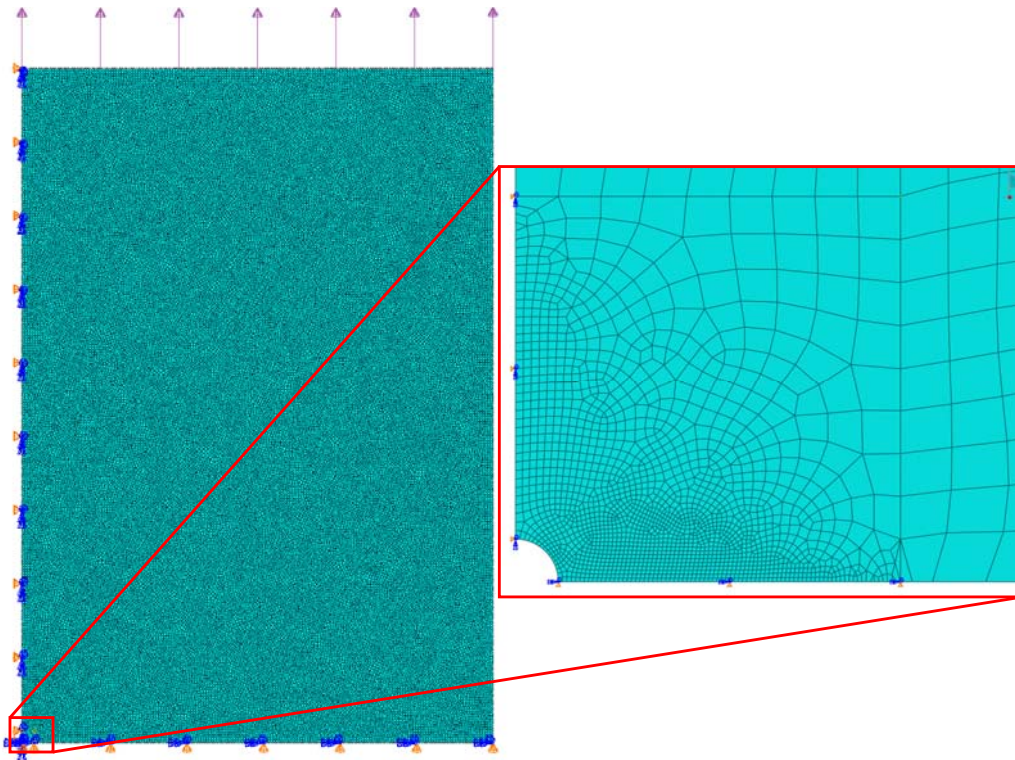
Fig. 4 Quarter Symmetry Model for 1-mm Hole Case
