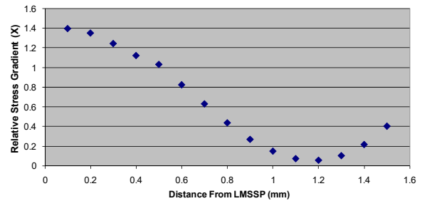
Fig. 8 Relative Stress Gradient for 2 mm Case
