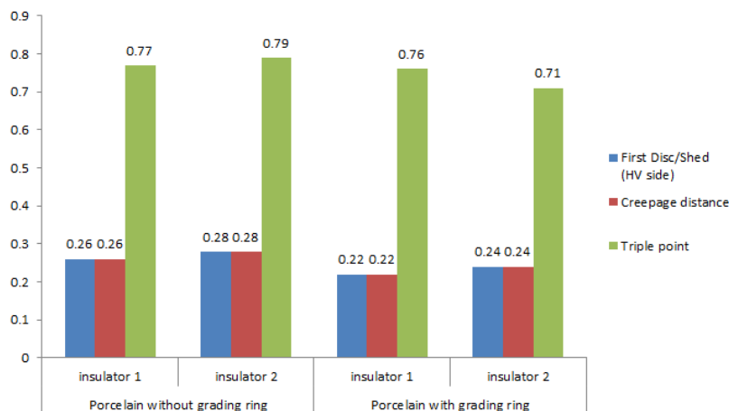
Fig. 11 Comparison between porcelain insulator with and without grading ring
