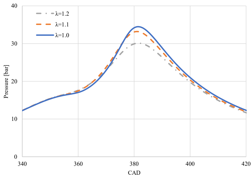
Fig. 5 In-cylinder pressure traces for the three conditions
