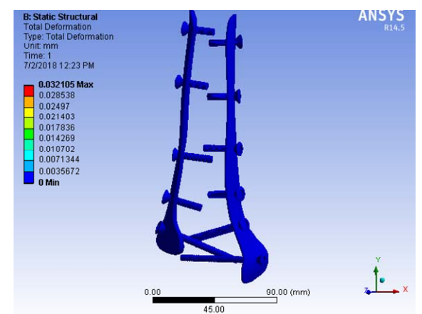
Fig. 9 (b) Total deformation variation in implant and screw
