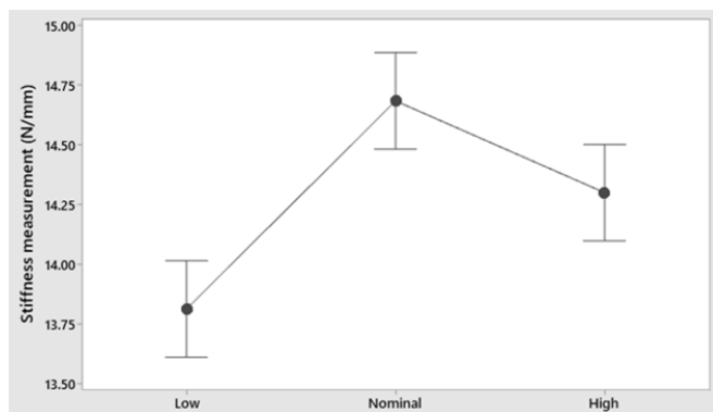
Fig. 9 Interval plot of TPB test 2
