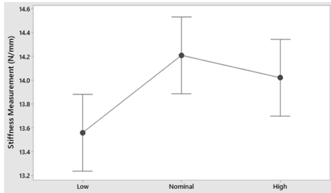
Fig. 8 Interval plot of TPB tests 1
