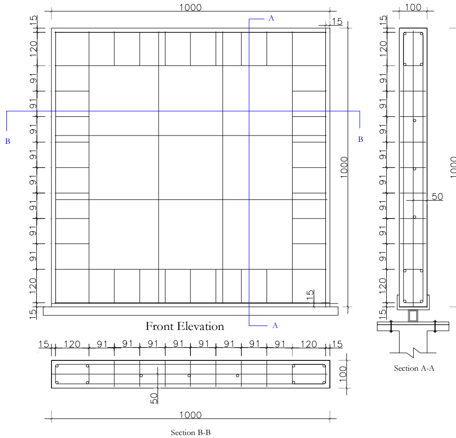
Fig. 1 Reinforcement cage
