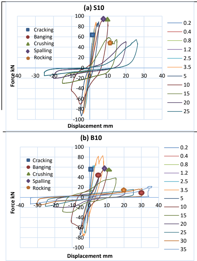
Fig. 7 Lateral force versus top-displacement relationship for S10 and B10 samples
