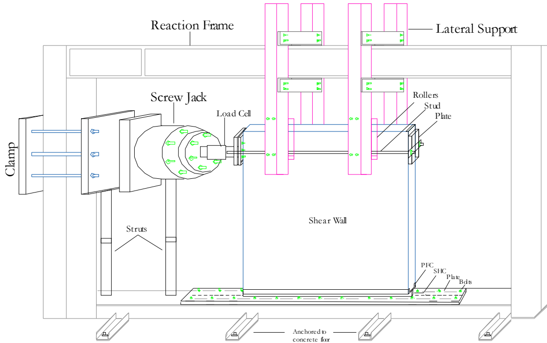
Fig. 3 Experimental test set up
