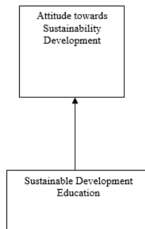
Fig. 1 Research Model
