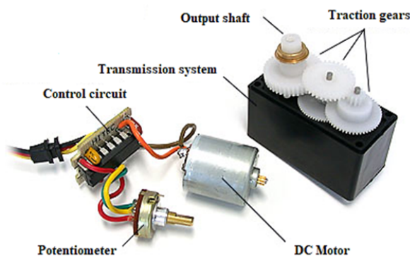
Fig. 6 Representation of the components that make up a servomotor, adapted from [11]
