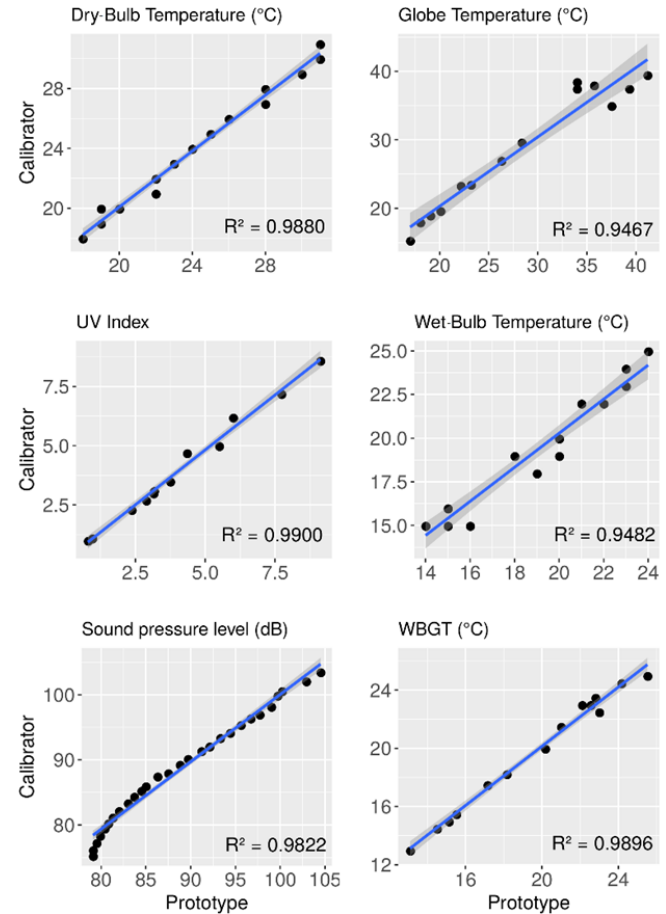
Fig. 2 Correlation plots between prototype and calibrator for environmental variables directly and indirectly measured with dedicated electronic modules: The correlation of determination ( R^2 ) between measurements is shown in the bottom right corner and ranged from 0.95 to 0.99. Generated using ggplot.
