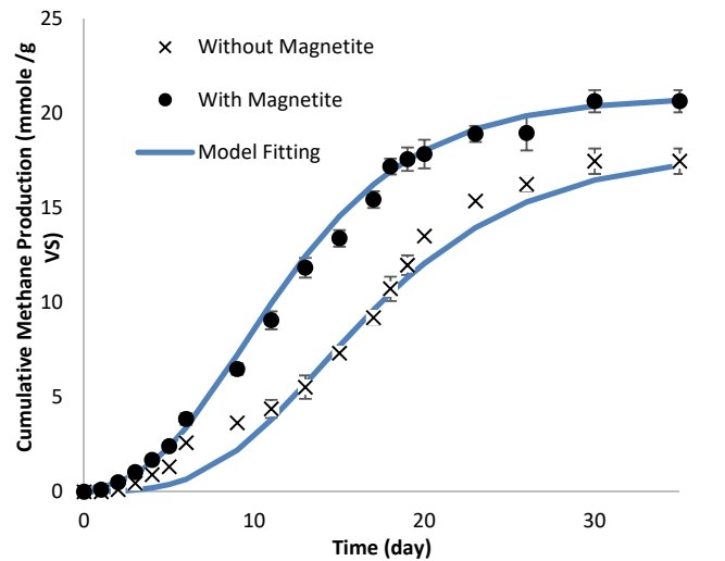
Fig. 1 Evolution of experimental and modelled methane production. Error bars represent the standard deviation of triplicate experiments
