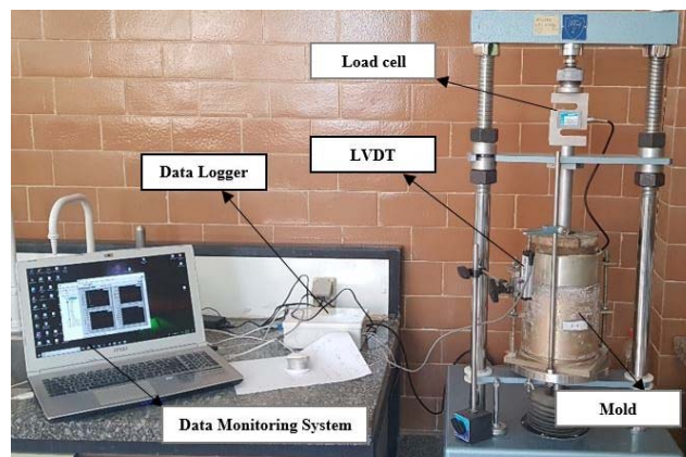
Fig. 10 Overview of the testing apparatus
