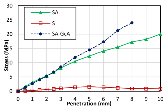
Fig. 12 Comparison of the stress-settlement behavior of geocomposite type A with unreinforced condition
