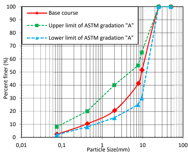
Fig. 6 Grain size distribution of base course material
