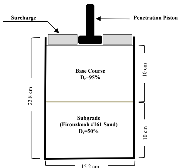
Fig. 9 Schematic representation of testing apparatus
