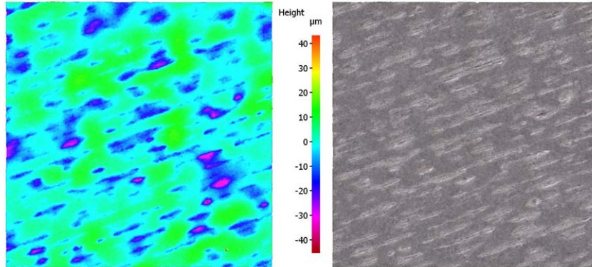
Fig. 3 Tumbling
