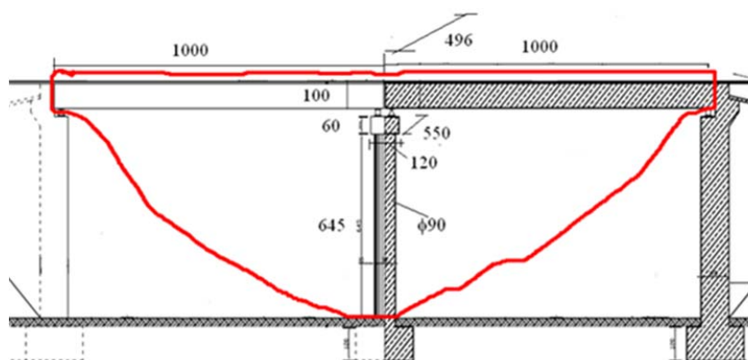
Fig. 2 Dimensions of analyzed part of concrete bridge
