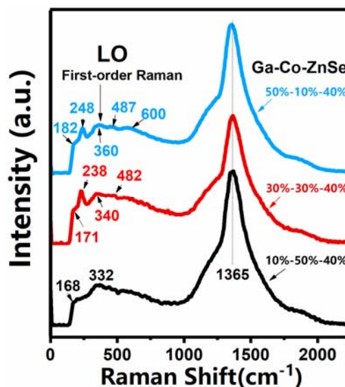
Fig. 2 Raman spectra of the Ga-Co-ZnSe ceramic bulks
