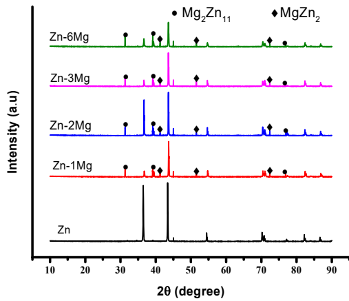
Fig. 4 XRD pattern of Zn-Mg alloy
