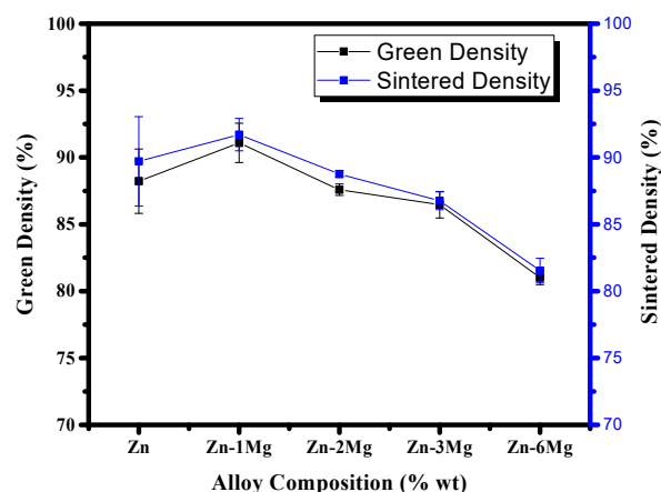
Fig. 2 Green and sintered densities of Zn-Mg alloys
