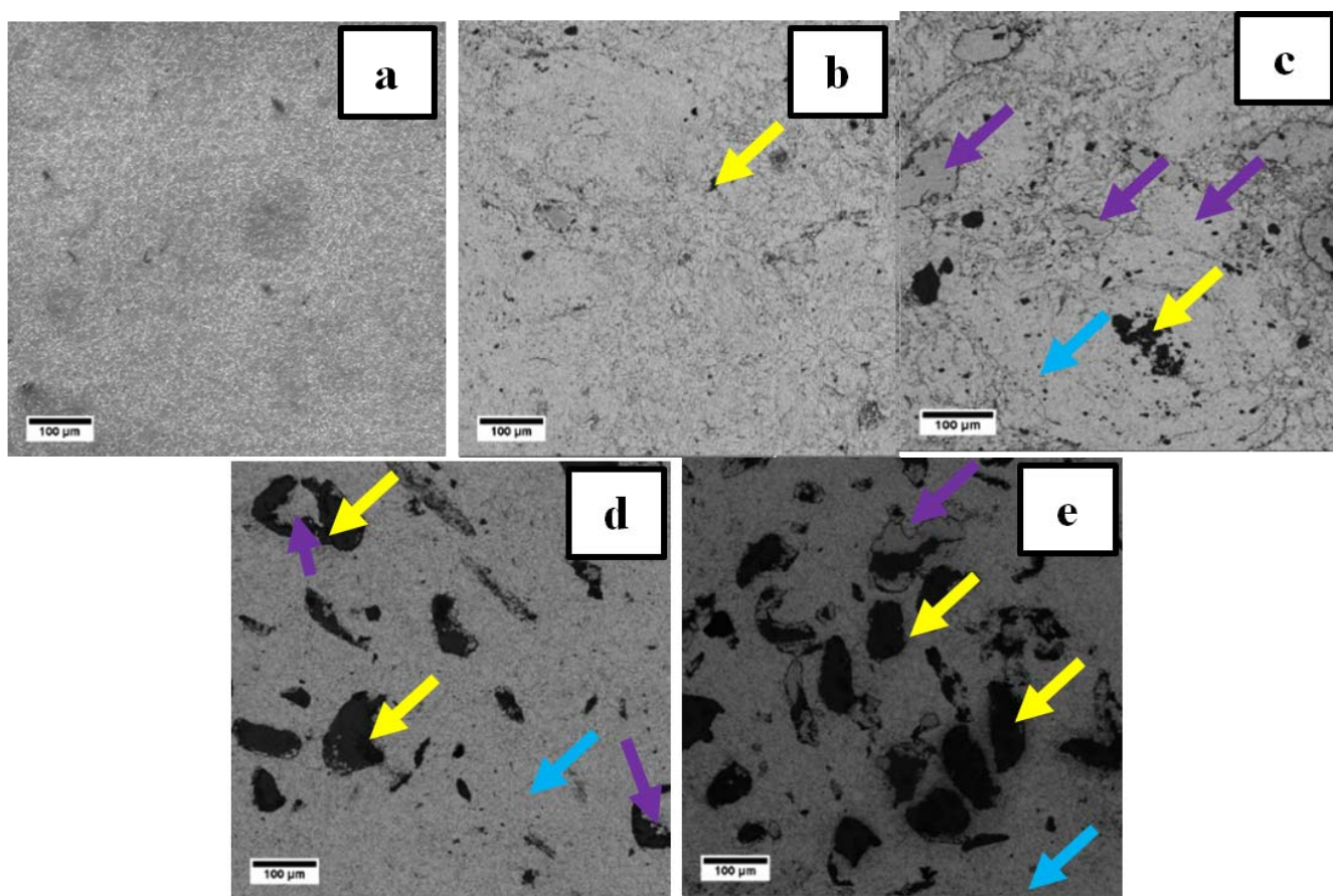
Fig. 3 Microstructure of Zn-Mg alloys
