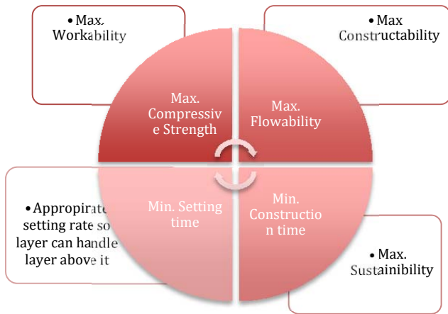
Fig. 1 Challenges for 3D Printing Concrete Mix
