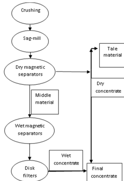
Fig. 1 Schematic presentation of iron Concentration Plant
