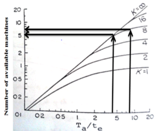
Fig. 4 Number of available machines base on rate T_a to t_c [18]
