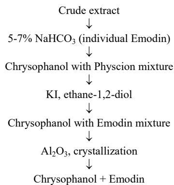
Fig. 1 Scheme of selective extraction of natural anthraquinones
