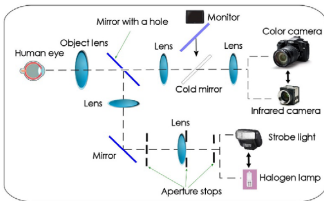
Fig. 4 Ophthalmological examination apparatus
