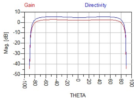
Fig. 6 Gain and directivity for 2.6 GHz
