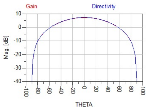
Fig. 7 Gain and directivity for 3.5 GHz
