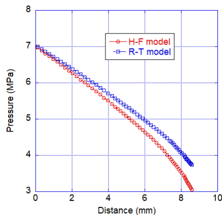
Fig. 2 Pressure distribution in 4 inch pipe crack
