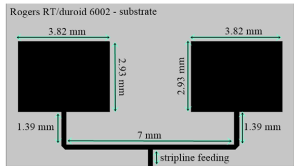
Fig. 5 A 2X1 Microstrip Antenna Array
