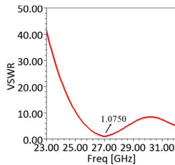
Fig. 7 VSWR plot for 2X1 antenna array
