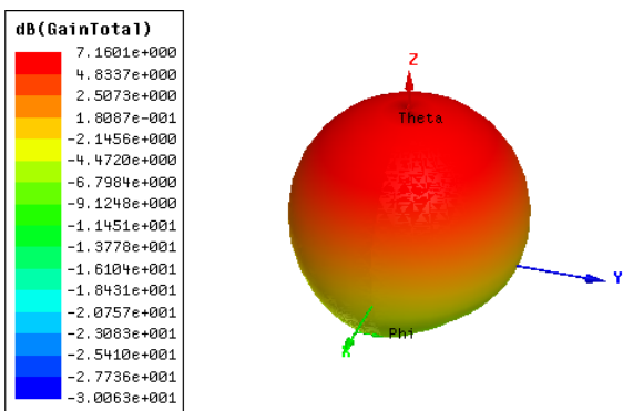
Fig. 4 3D Gain plot for Conventional Antenna
