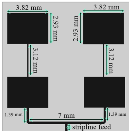
Fig. 9 A 4 – Element Corporate Series Feed Antenna Array
