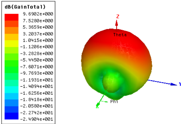
Fig. 8 3D gain plot for 2X1 antenna array
