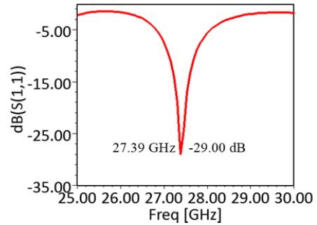
Fig. 10 S11 plot for the 4 – Element Corporate Series Feed Antenna Array
