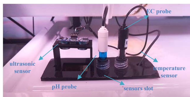
Fig. 6 Water tank sensors hosting kit
