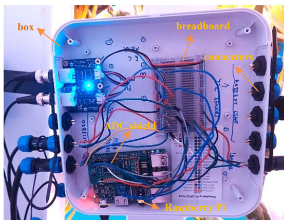
Fig. 2 Monitoring System – Hardware
