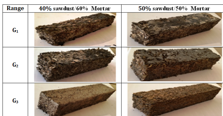
Fig. 2 Reinforced mortar specimens of different ranges
