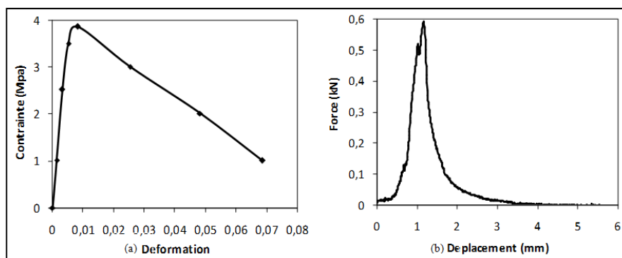
Fig. 3 Stress-strain curves
