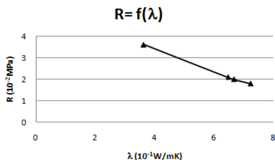
Fig. 6 Resistance curve as function of thermal conductivity
