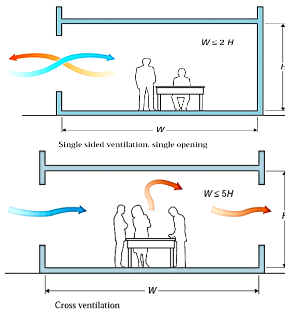
Fig. 2 Basic forms of ventilation strategy, (CIBSE AM10 and CIBSE Guide F)
