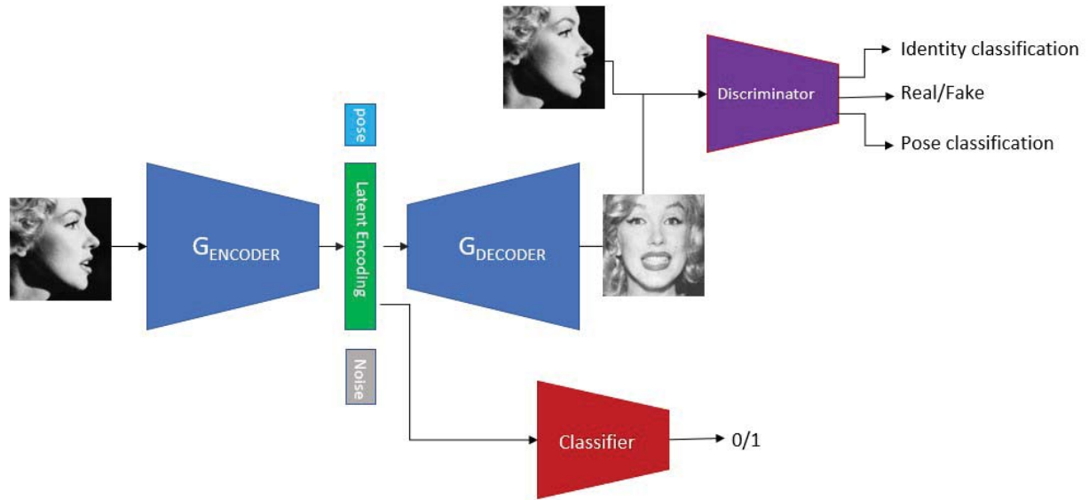
Fig. 2 Overall architecture the proposed framework. It fulfills two purposes: 1) learning a standalone identity representation. 2) synthesis of frontal from the disentangled representation
