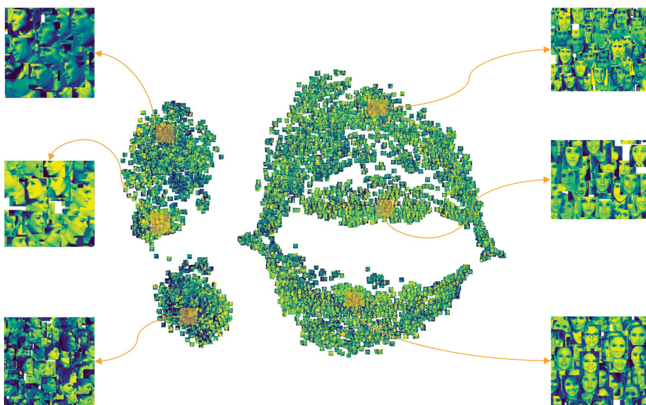
Fig. 5 Two-dimensional projection of Latent space. Different colour represents a different identity. Profile faces are grouped differently than frontal faces. Face image for one identity is shown
