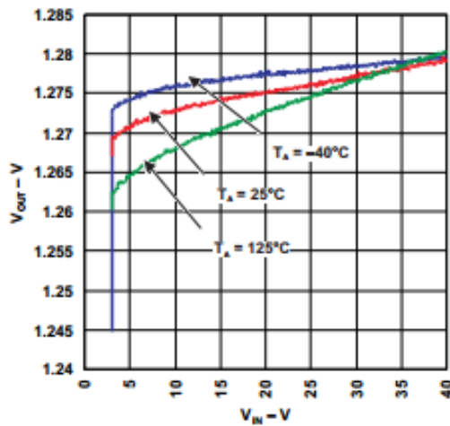
Fig. 8 Line regulation
