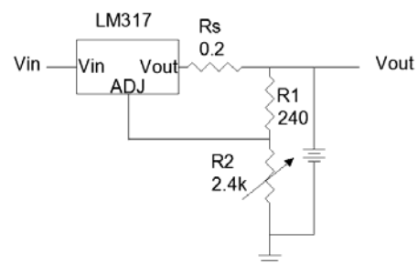
Fig. 7 Typical voltage regulator circuit
