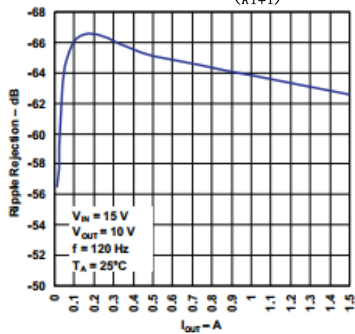
Fig. 9 Ripple rejection
